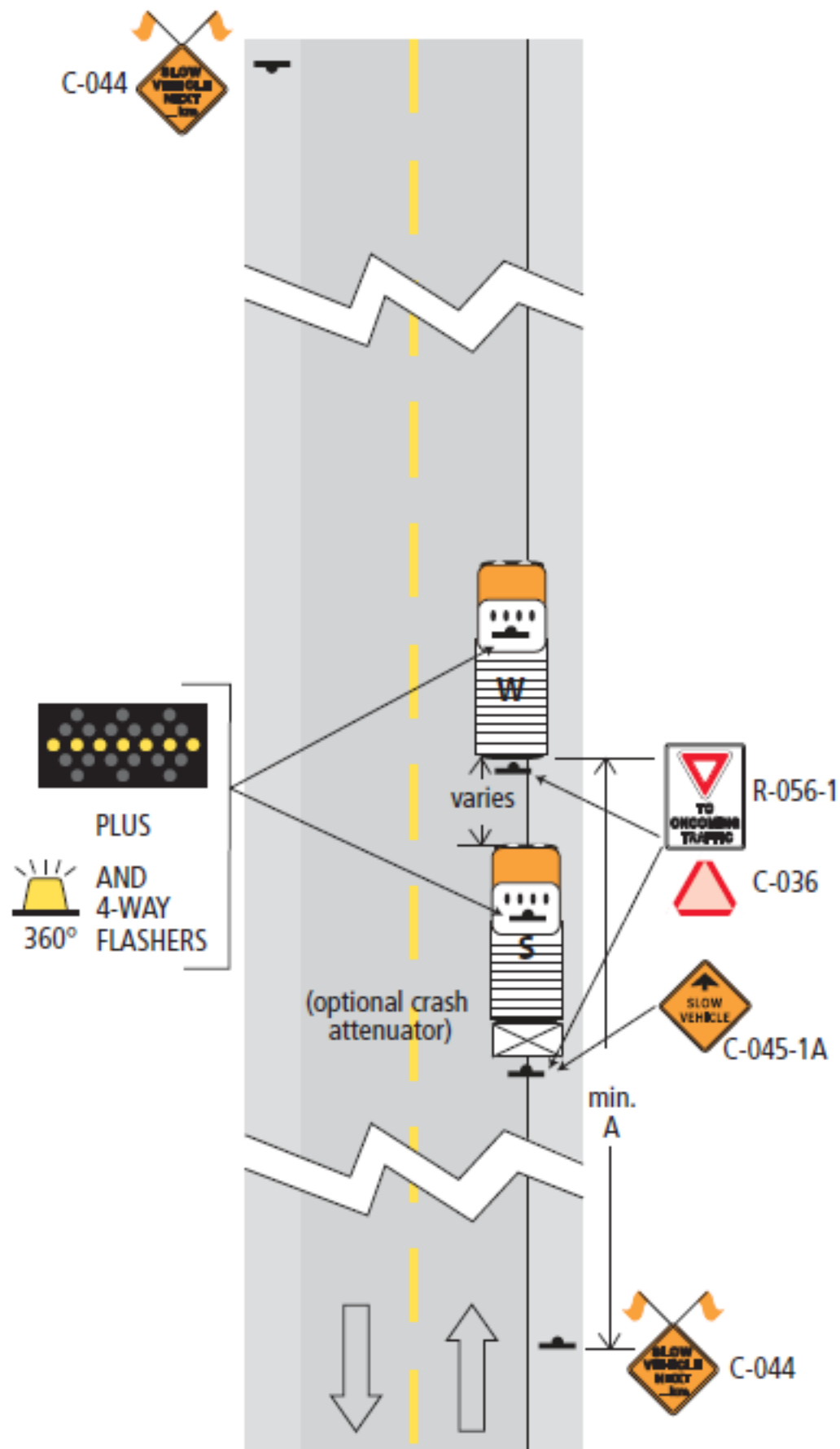
Figure 10.2: Continuously Slow-Moving Work – Two-Lane, Two-Way Roadway
